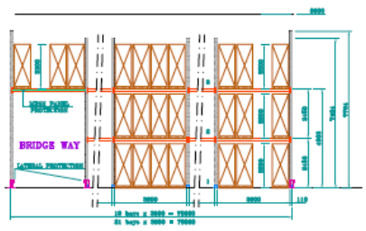
Type A -pallets height 2200 Racks 1S, 1D, 2D, 3D, 4D, 5D & 7D
