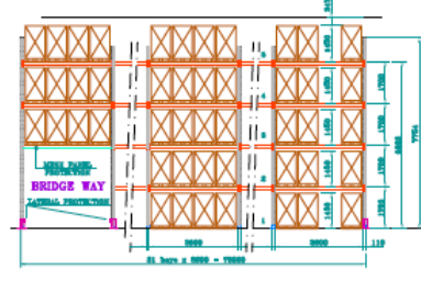
Type D -pallets height 1450- Racks 13D, 14D, 15D, 16D, 17D, 18D & 19D
