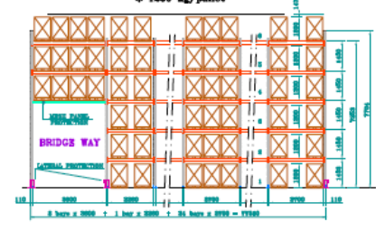
Type E -pallets height 1200- Rack 20D * 1200 kg/pallet
