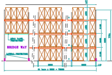
Type B -pallets height 1850- Racks 8D, 9D, 10D, 11D & 12D
